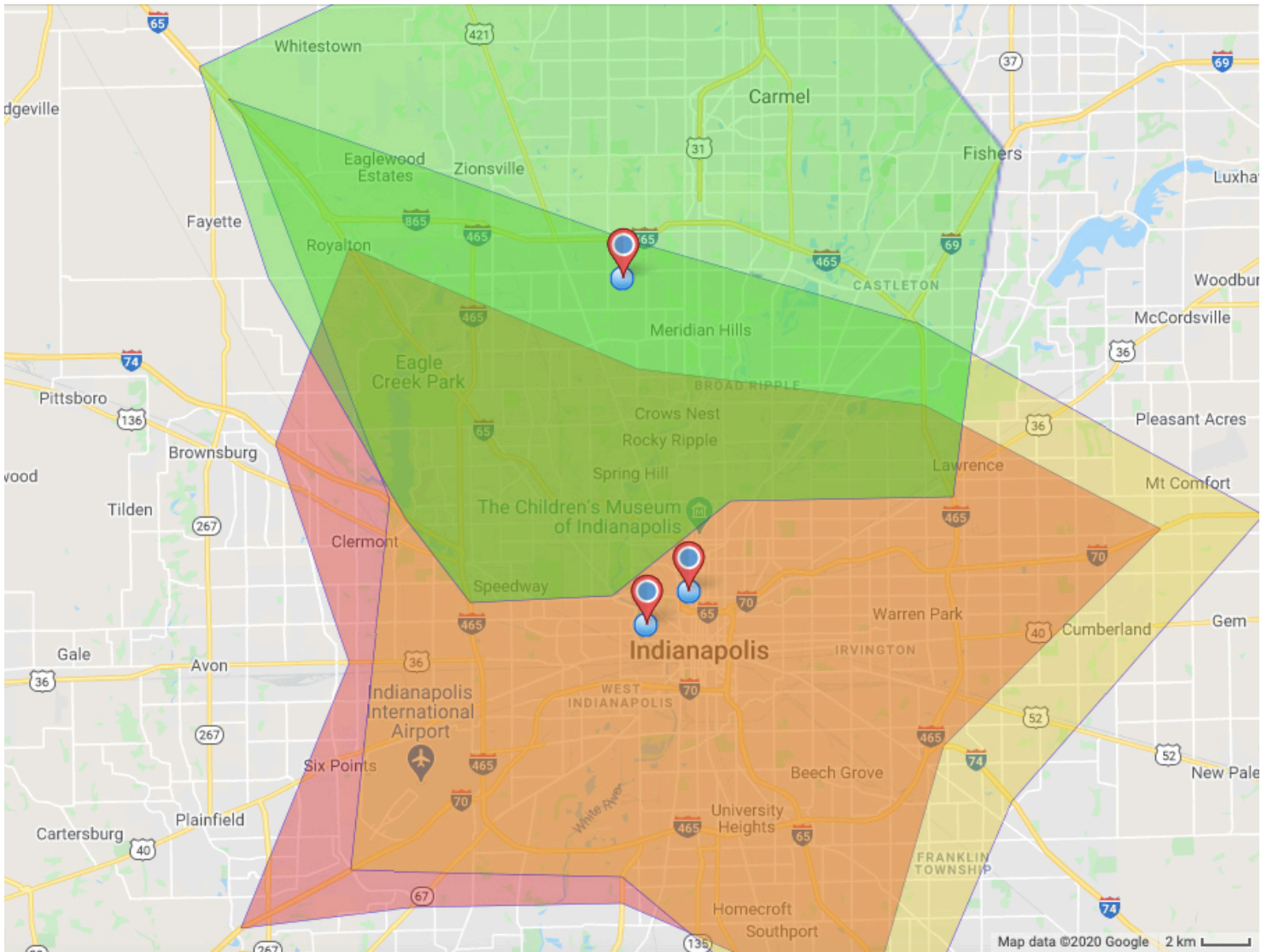
Supplemental Material 6: Indianapolis Trauma Center Density Plots the level 1 and 2 trauma centers in Indianapolis the US. Colored Polygons represent 20-minute drive radius of the level 1 trauma centers.
